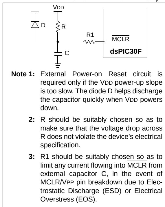
FIGURE 20-6: EXTERNAL POWER-ON RESET CIRCUIT (FOR SLOW V_{DD} POWER-UP)
